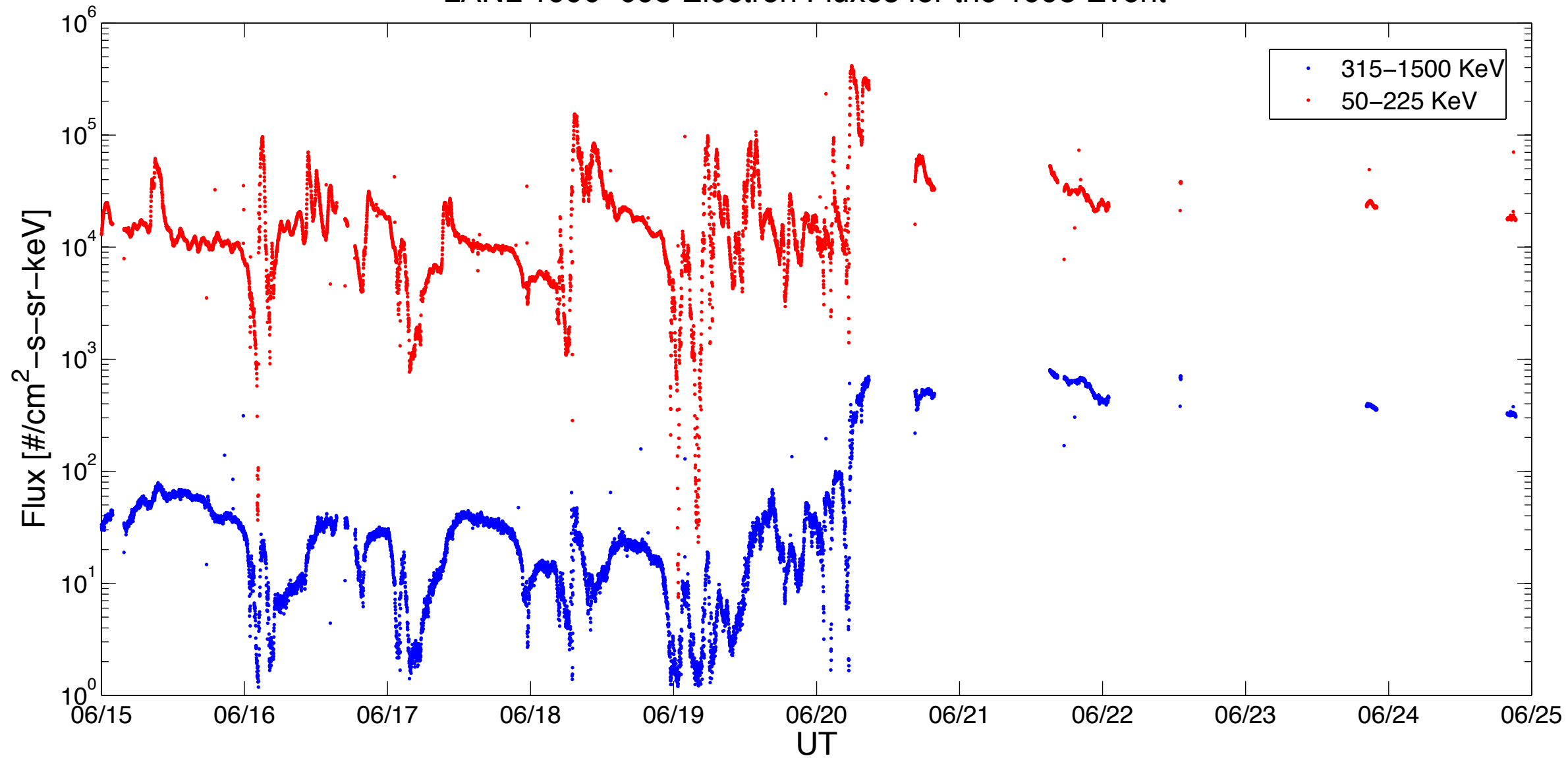
LANL 1990–095 Electron Fluxes for the 1995 Event
